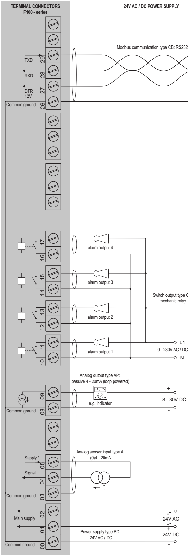
Configuration example F190-P-AP-CB-OS-PD-XX-ZX
