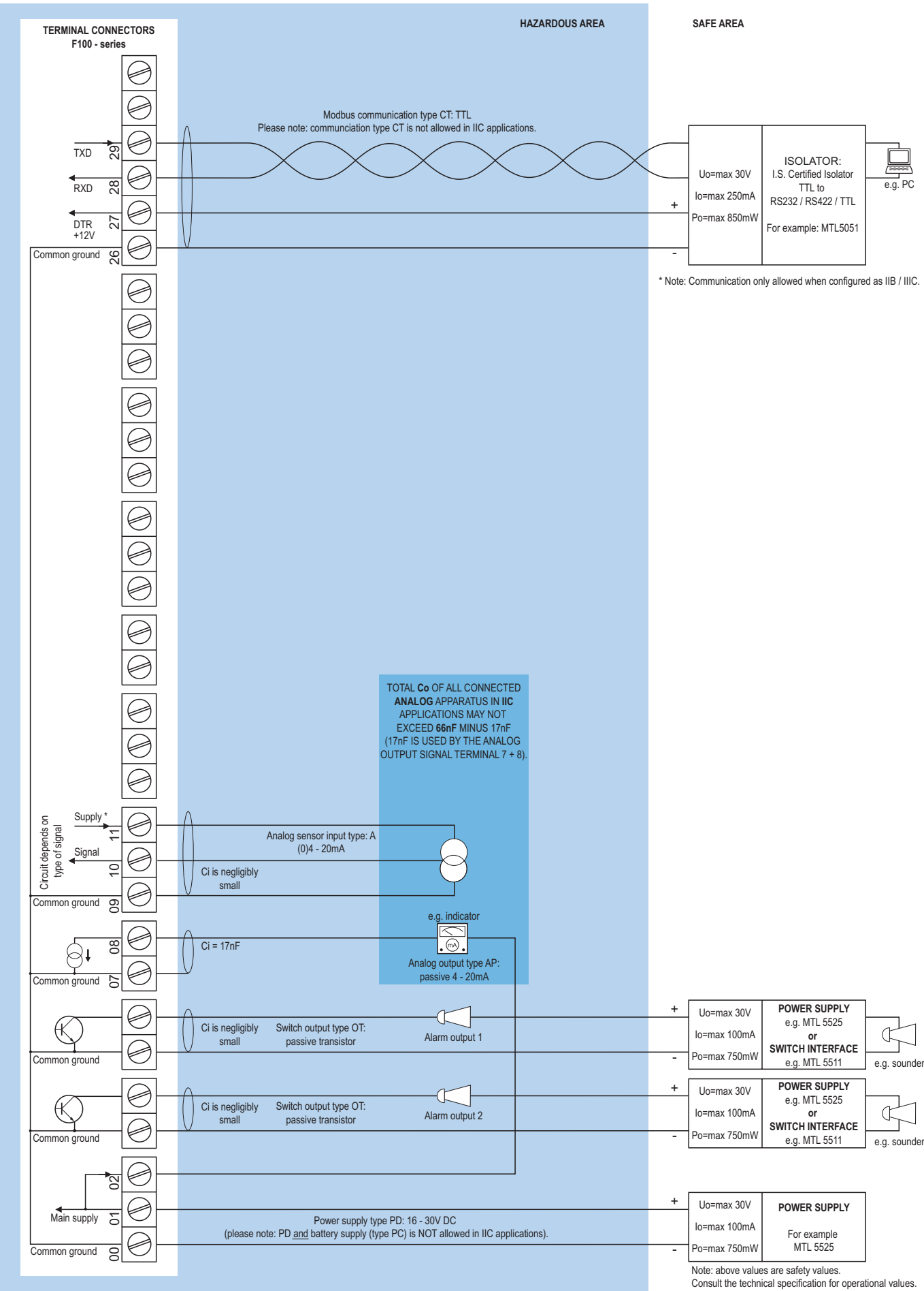
Configuration example IIB / IIIC and IIC - F190-A-AP-(CT)-OT-PD-XI - Power requirement 16 - 30V DC
